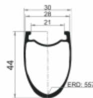
AIRSPEED44
